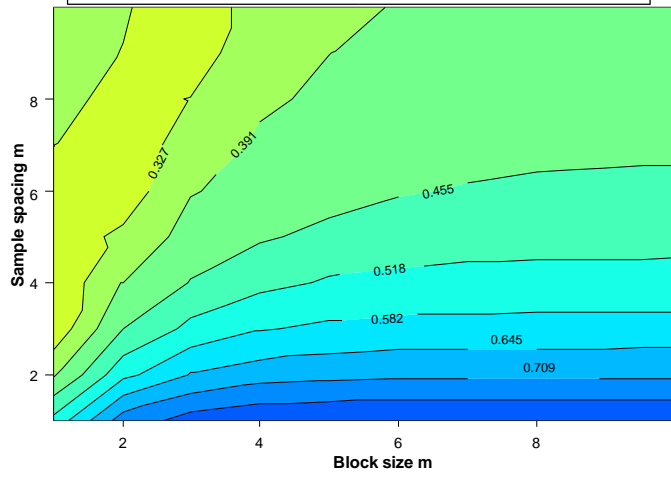
OSSFIM: Contour plot of kriging variances as function of sample spacing and block size
